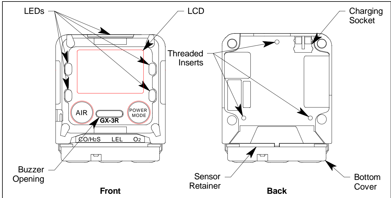
Figure 1: Component Location
