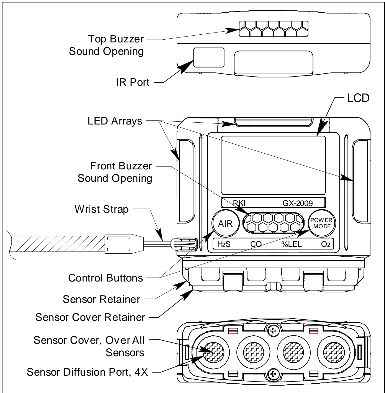
Figure 1: Top, Front & Bottom Views
